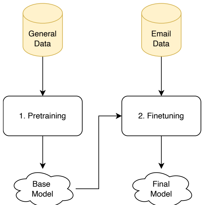
Figure 23: Two-stage training strategy
