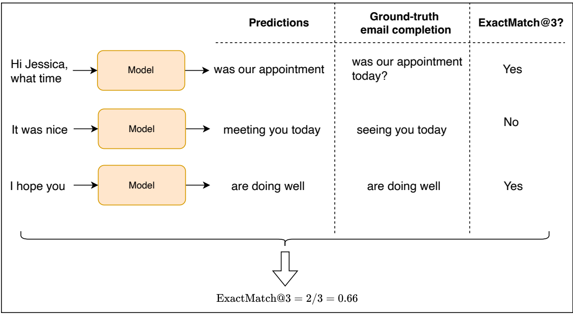
Figure 39: Example of calculating ExactMatch@3 for three sequences
