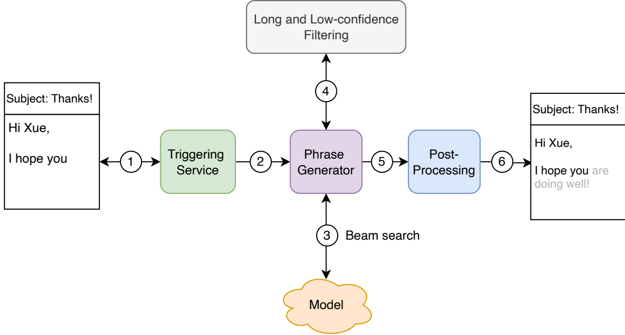
Figure 43: Smart Compose feature overall design
