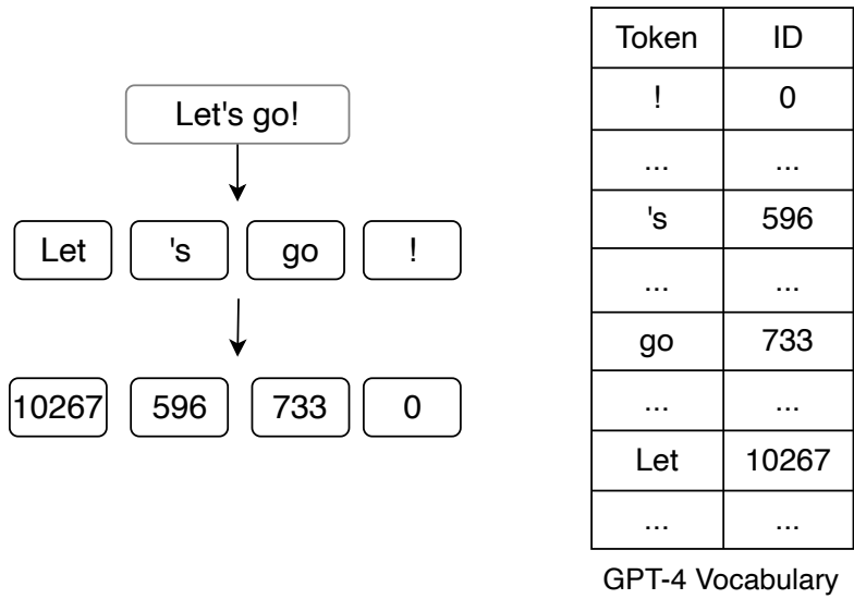
Figure 10: Example of token indexing
