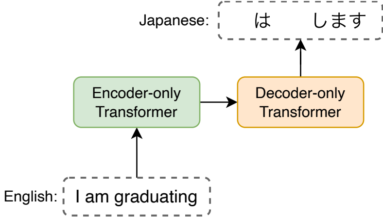
Figure 13: Encoder-decoder Transformer used for language translation
